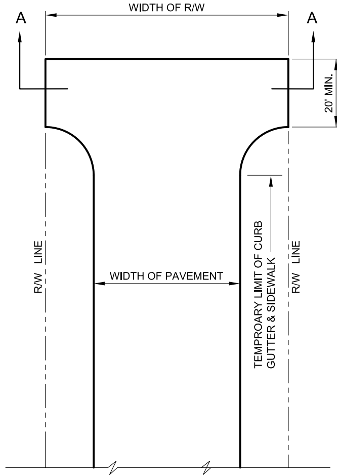
PLAN
