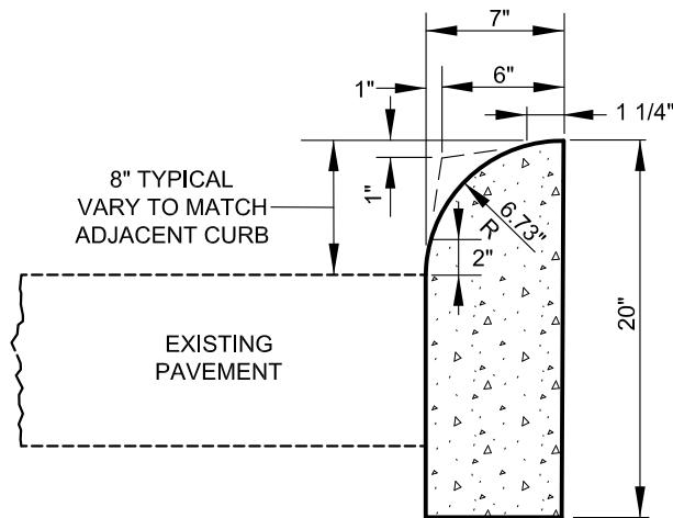
BC TYPE 'A' MODIFIED CURB
