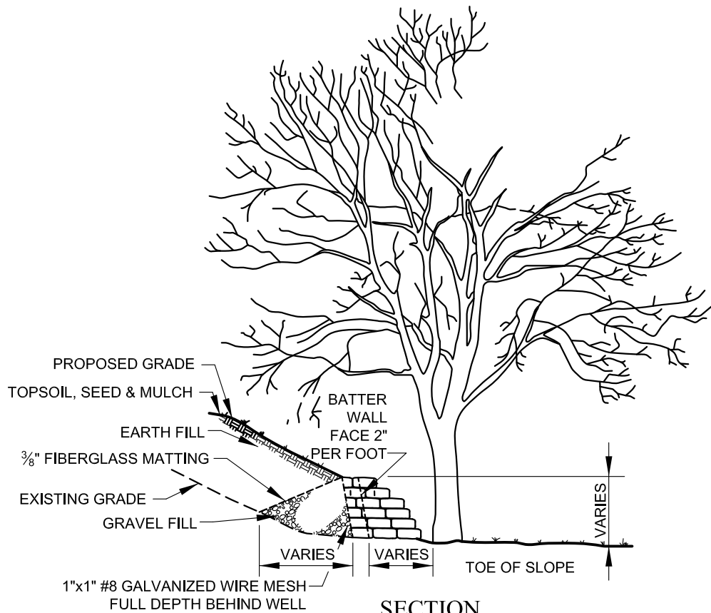
SECTION
