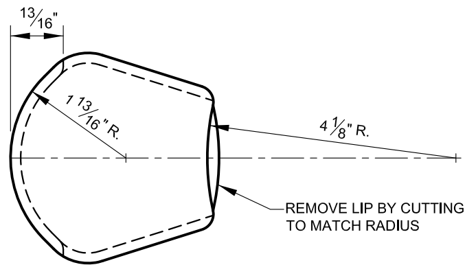
BOLT COVER DETAIL
